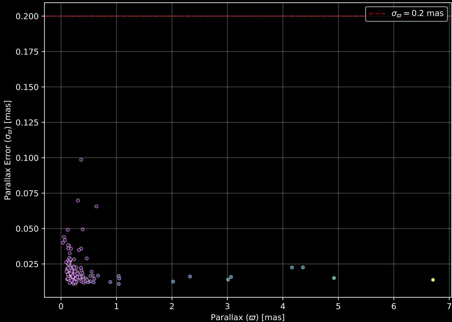
APOGEE DR17 Field: [Cas_N] Parallax Quality (n= 145)
