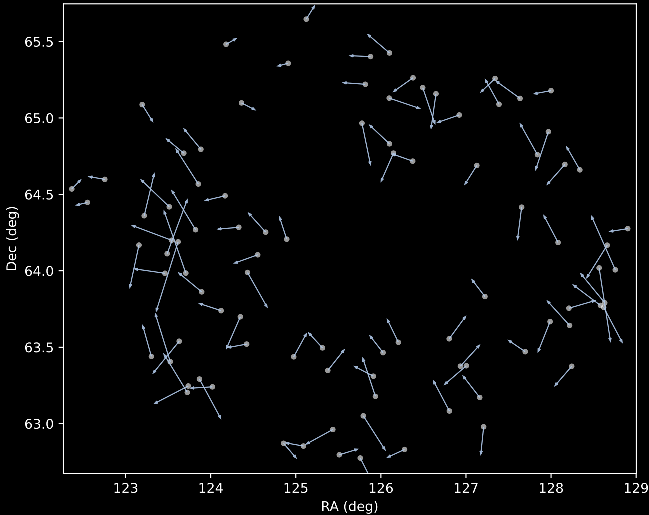
APOGEE DR17 Cluster 1 Proper Motion Vectors (n=93)
