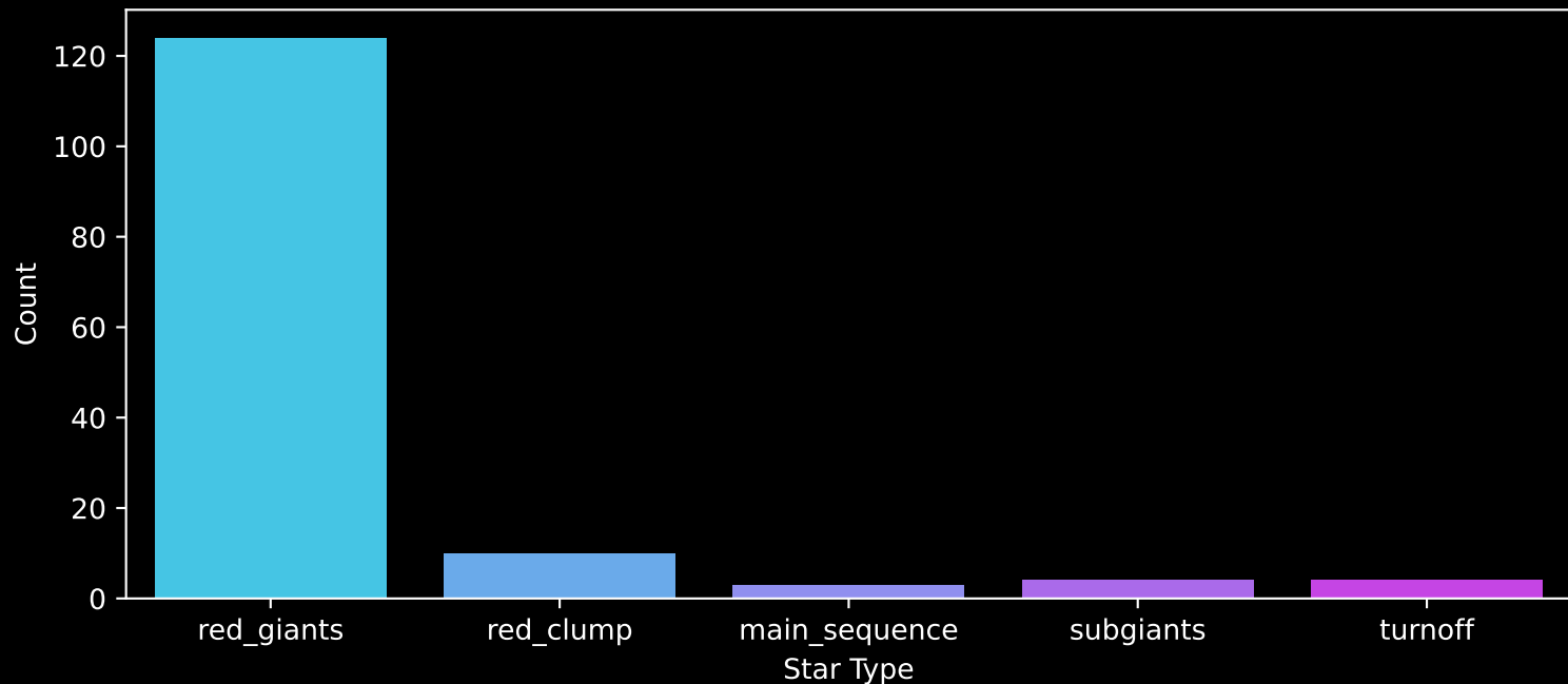
APOGEE DR17 Field: [Cas_N] Count plot of Star Type
