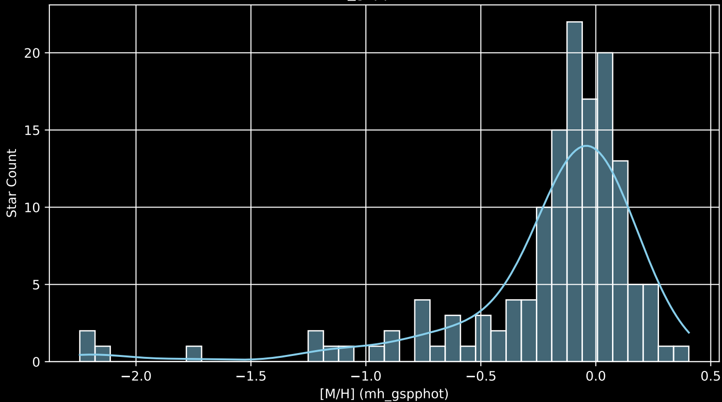
APOGEE DR17 Field: [Cas_N [M/H] (mh_gspphot) (n= 142)
