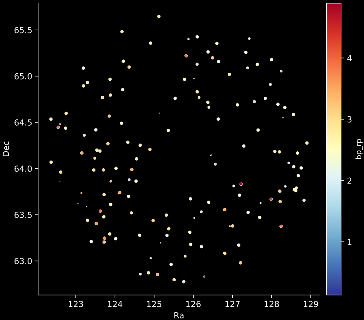
APOGEE DR17 Field: [Cas_N] Stars: 145
