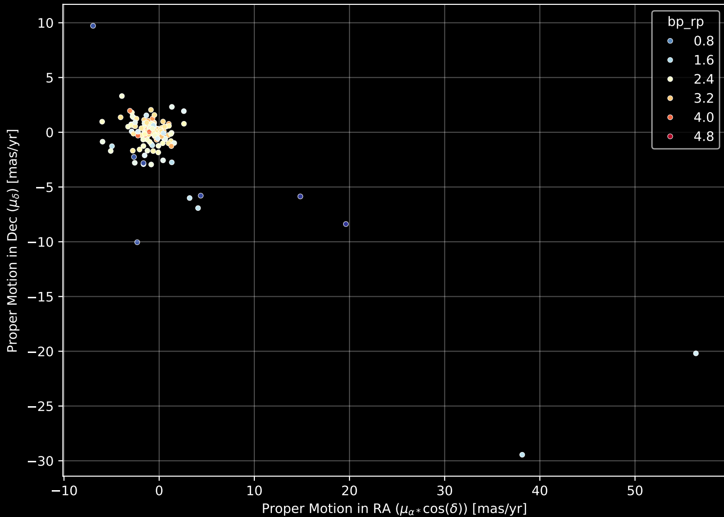
APOGEE DR17 Field: [Cas_N] Proper Motion Diagram (n= 145)
