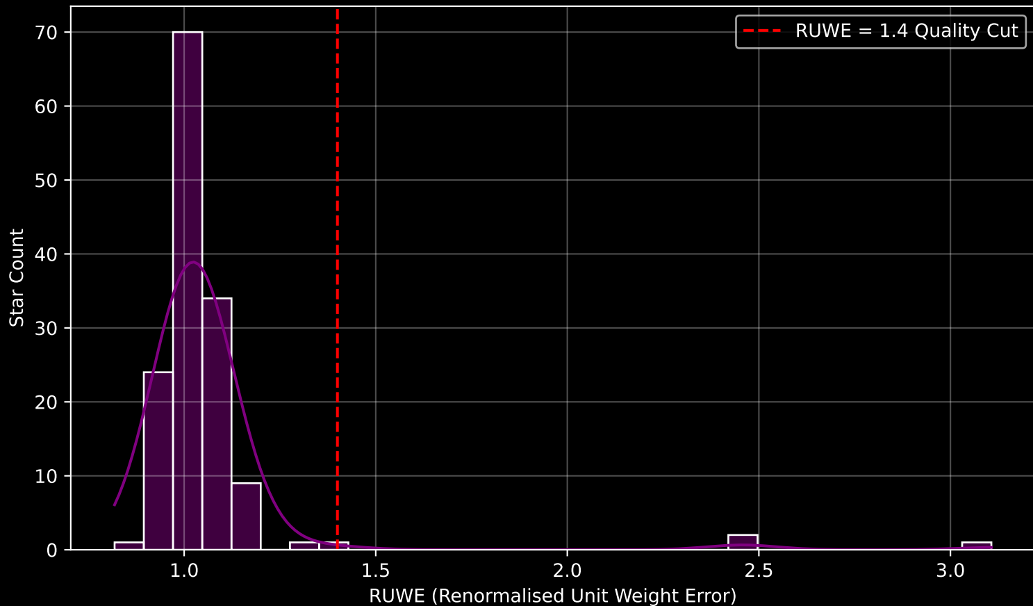
GAPOGEE DR17 Field [Cas_N] RUWE Distribution (n= 143)
